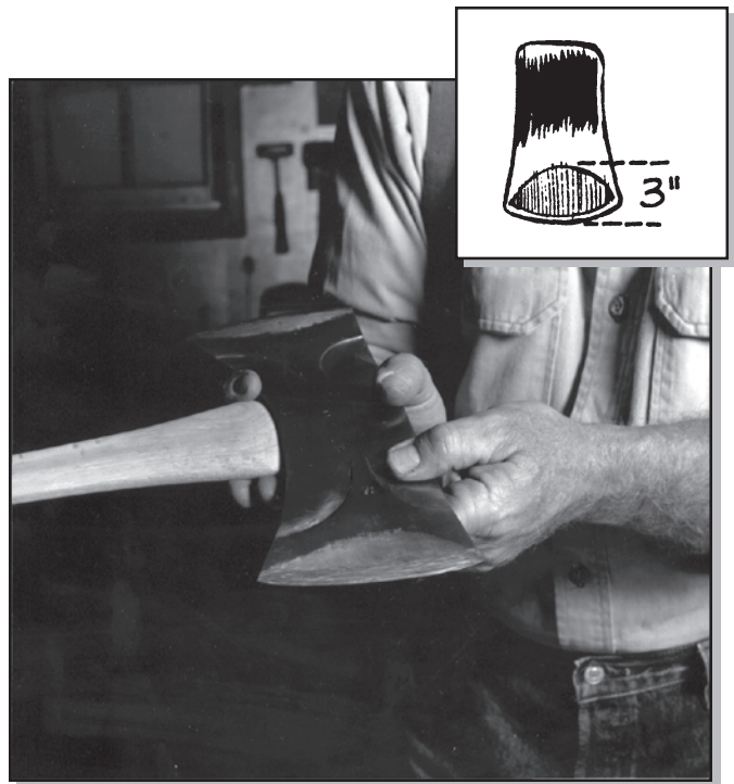
Figure 66—When sharpening, try for a fan-shaped effect on the cheek of the ax (drawing by Frederic H. Kock).
