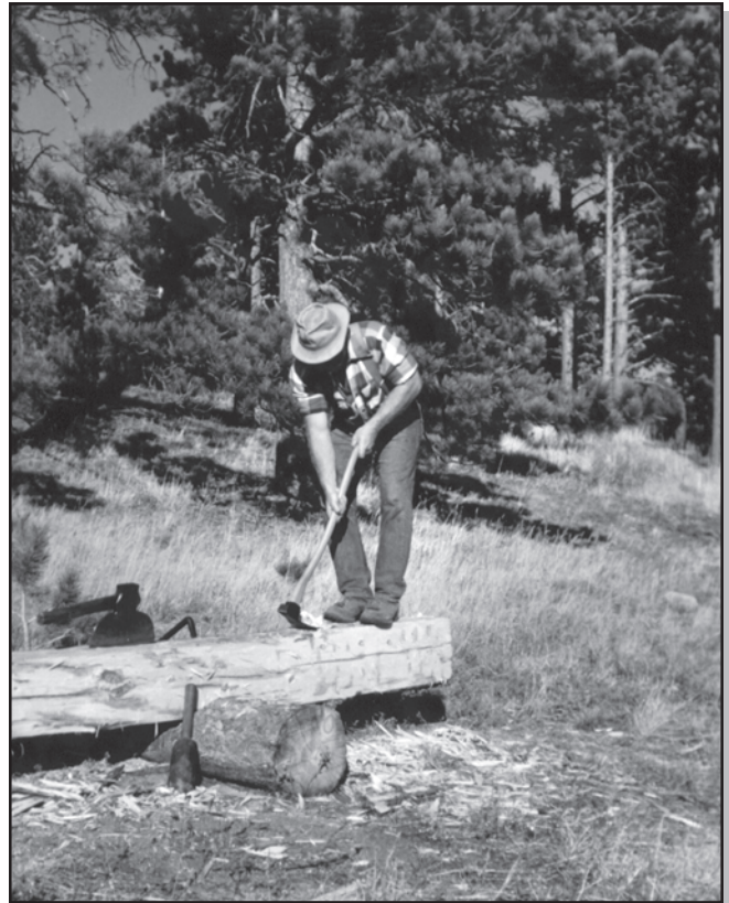
Figure 104—Adz work requires the utmost concentration to avoid cutting your feet.
